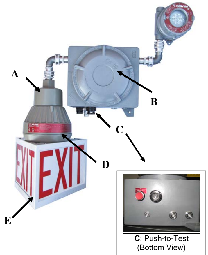
Figure 7: (Assembly of EBS System)
