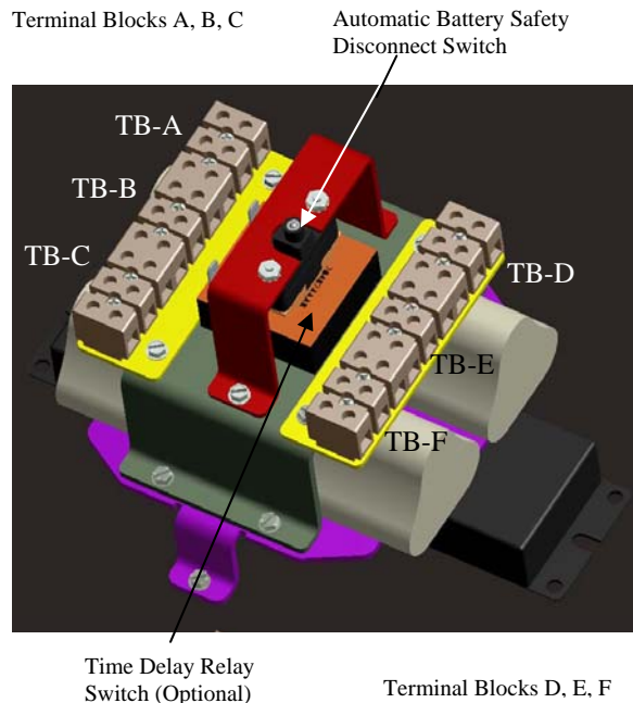
Figure 10: Internal Configuration of EBS System (Wired in Accordance with Figure 9: Field Wiring Schematics)
