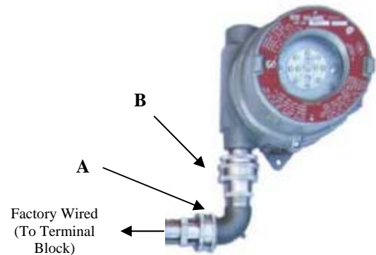
Figure 3: Adjustment of Unions on EBSHK1030 Head
