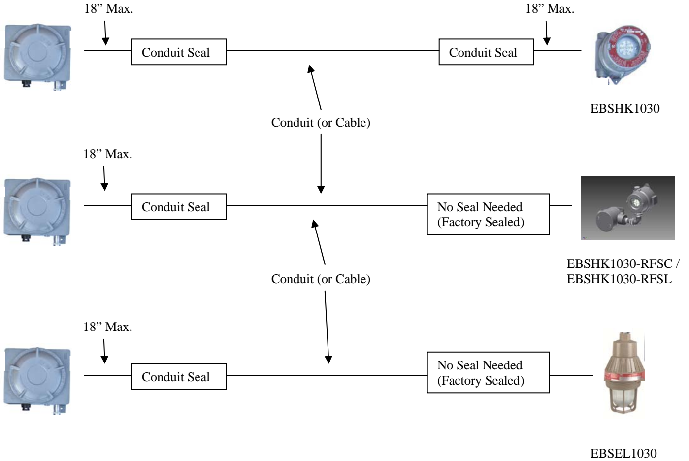
Figure 9: Sealing Requirements for Remote Luminaire Heads
